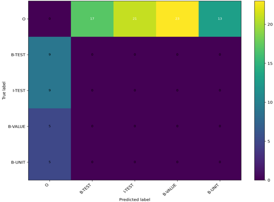
Misclassification-Only Heatmap
