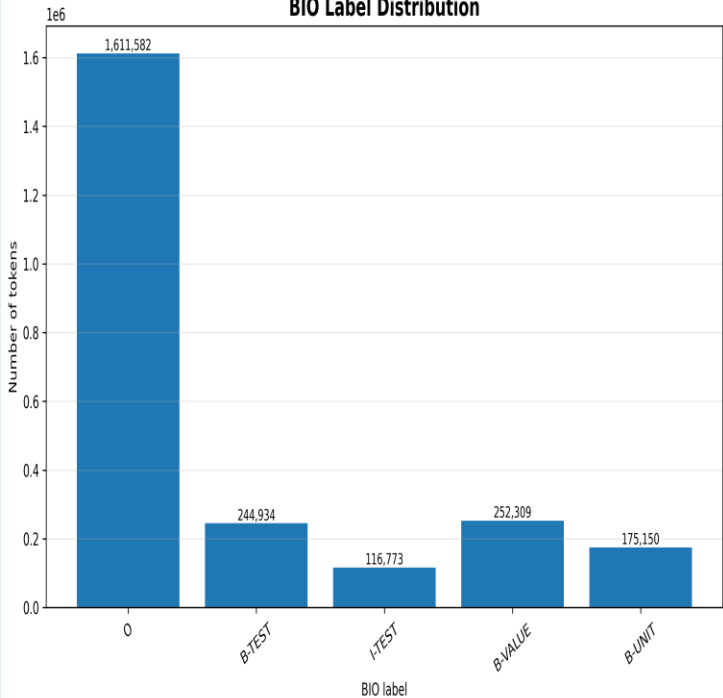
BIO Label Distribution
